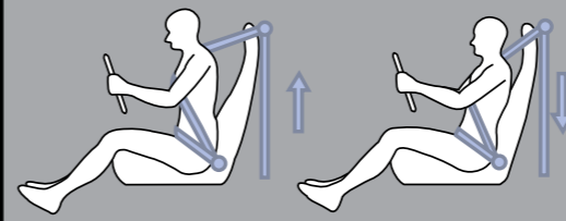
Front Seat Belts Pretensioner with Load Limiter
